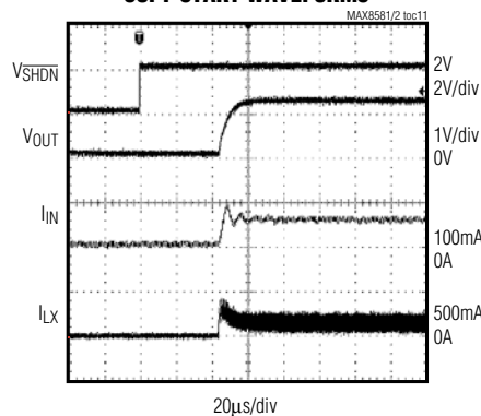
SOFT-START WAVEFORMS
