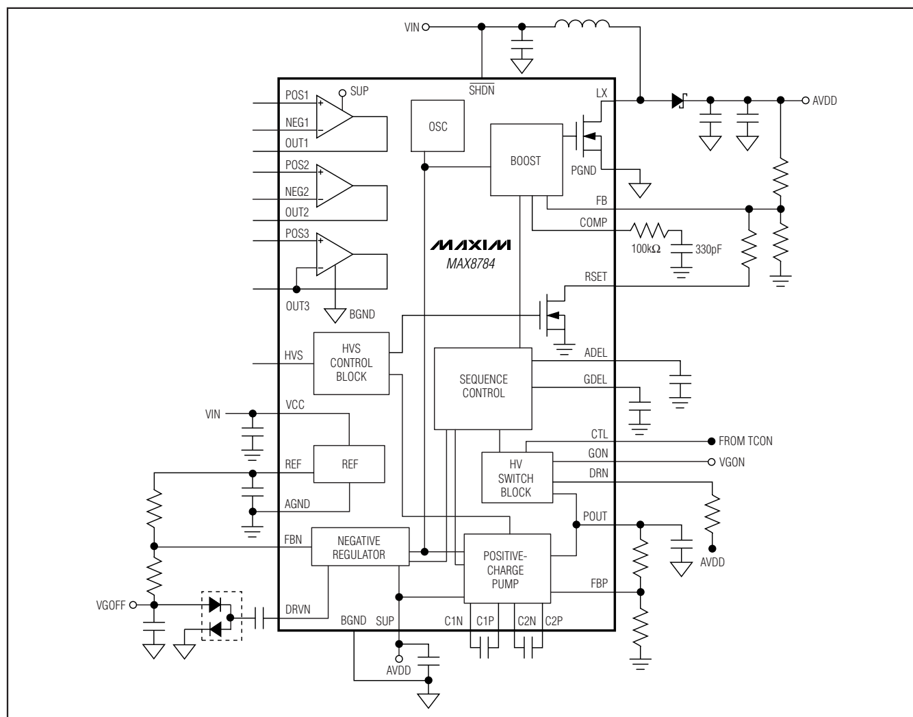
Figure 2. Functional Diagram
