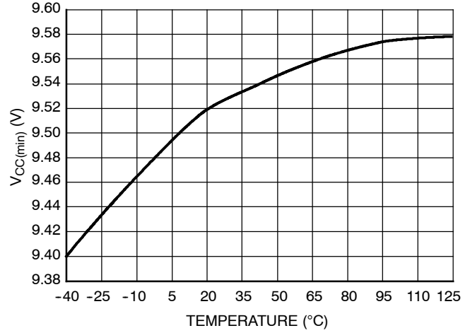
Figure 4. V CC(min)
