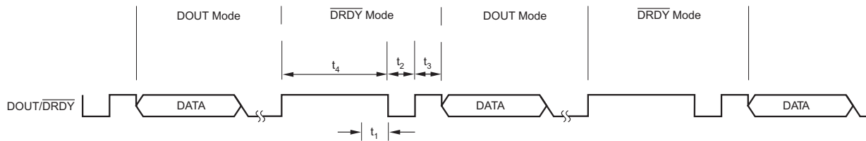
Figure 31. DOUT/DRDY Partitioning
