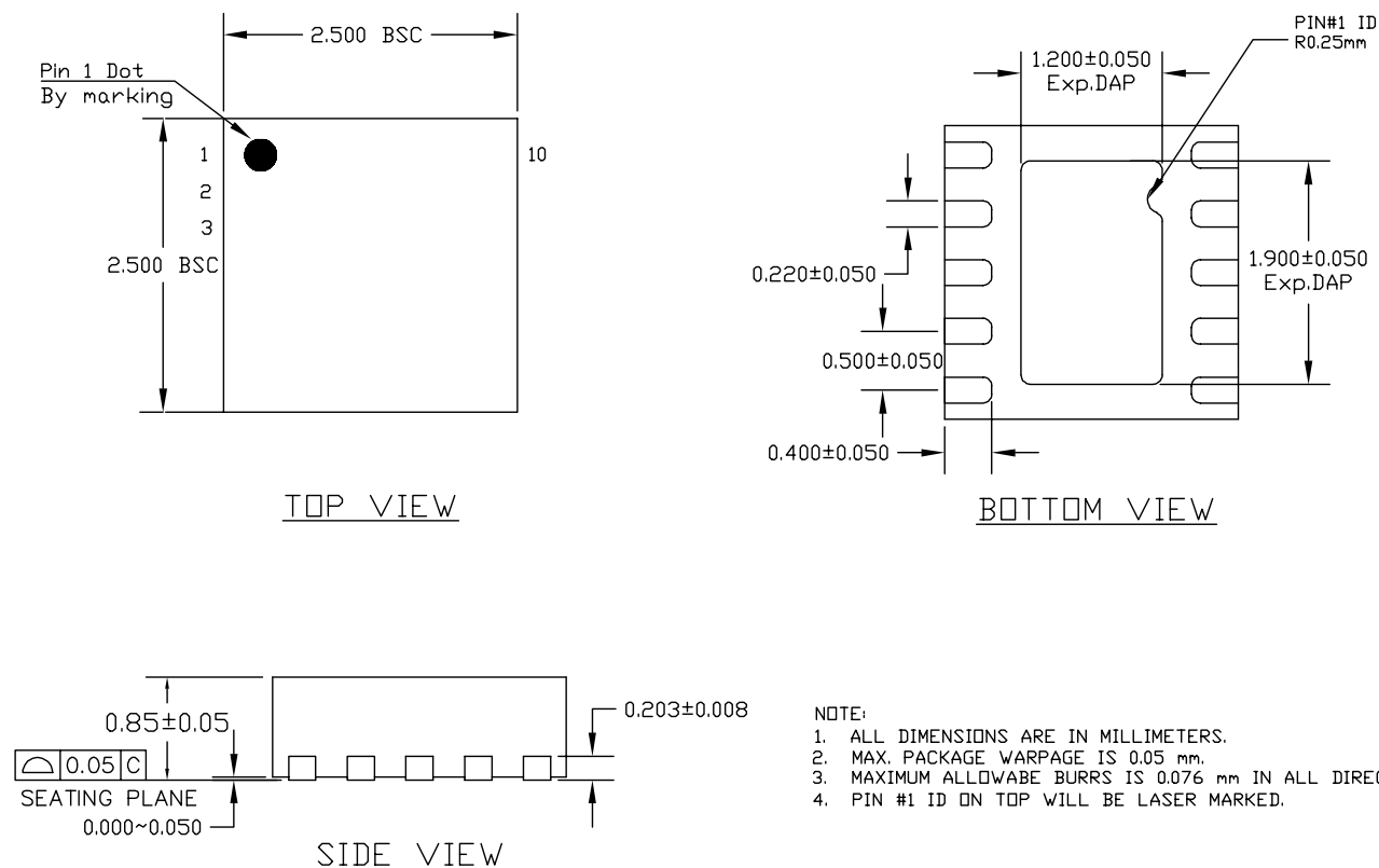
10-Pin Package MLF® (ML)
