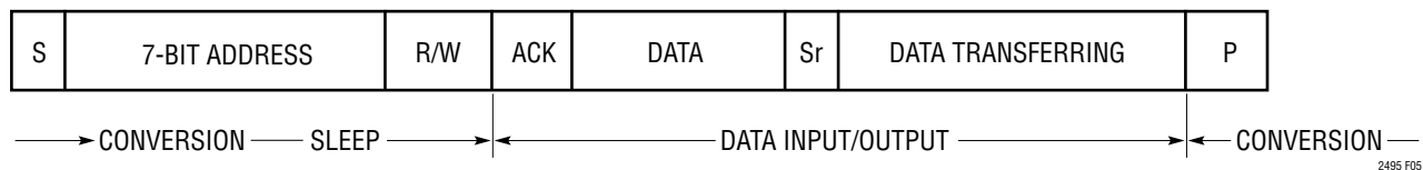
Figure 6. Conversion Sequence
