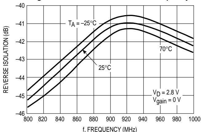
Figure 2. Reverse Isolation versus Frequency
