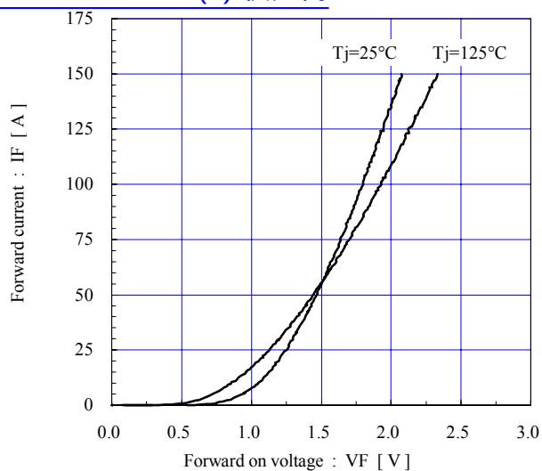
Forward current vs. Forward on voltage (typ.)
