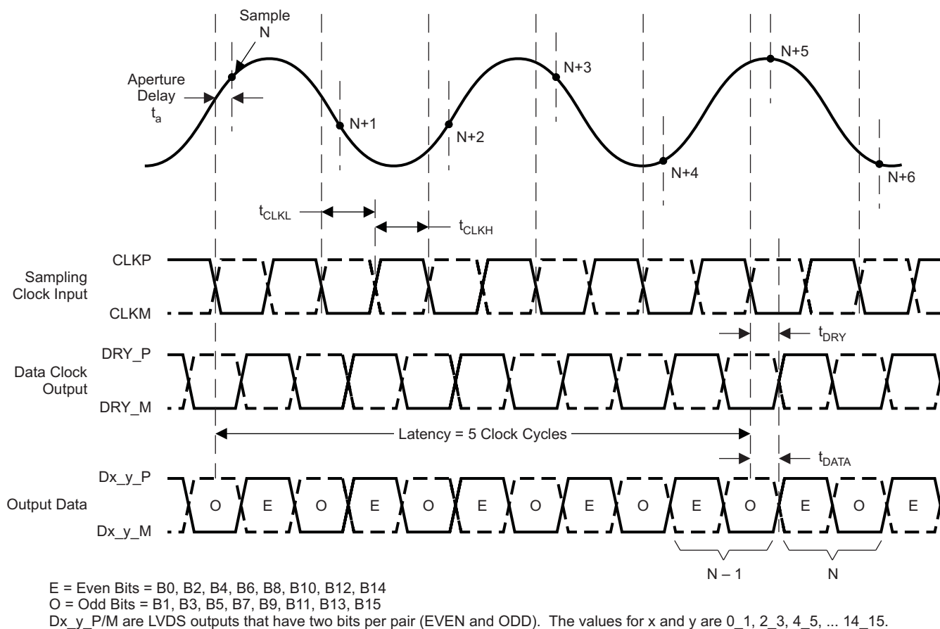
Figure 1. Timing Diagram
