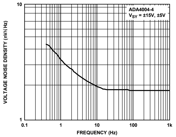
Figure 37. Voltage Noise Density vs. Frequency
