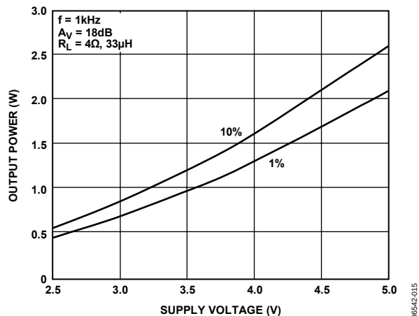
Figure 15. Maximum Output Power vs. Supply Voltage, R_L = 4\ \Omega , A_V = 18\ \text{dB}
