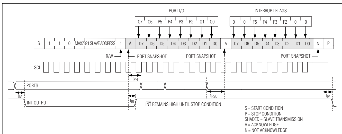
Figure 7. Reading the MAX7323 (2 Data Bytes)
