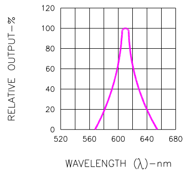
Fig.2 SPECTRAL RESPONSE
