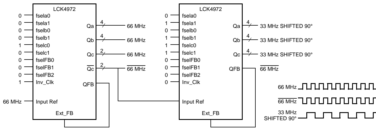
Figure 4-5. Phase Delay Example Using Two LCK4972s
