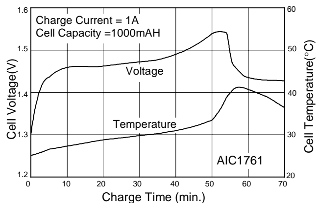
Fig. 7 Charge Characteristics of NiMH Battery
