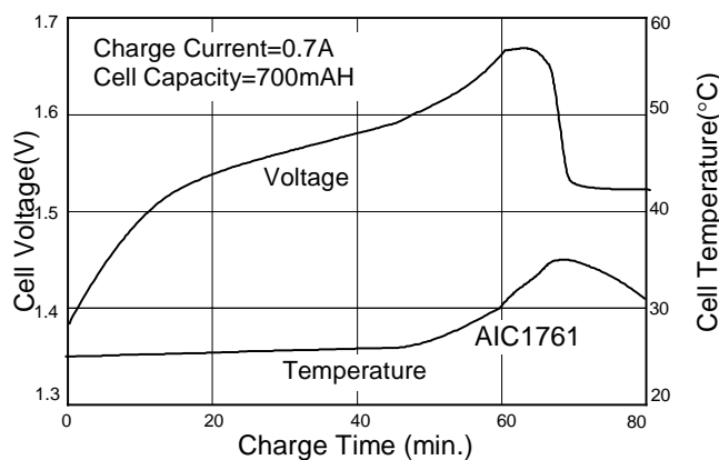
Fig. 8 Charge Characteristics of NiCd Battery
