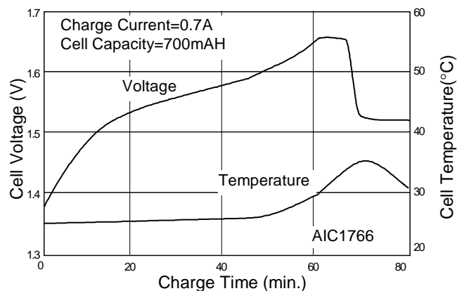
Fig. 6 Charge Characteristics of NiCd Battery
