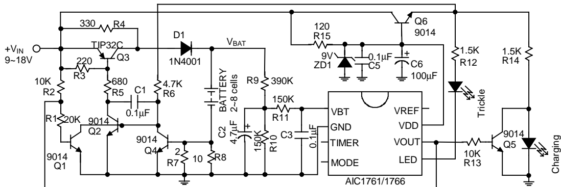
FIG. 12 Step-Up/Down Rechargeable Battery Charger
