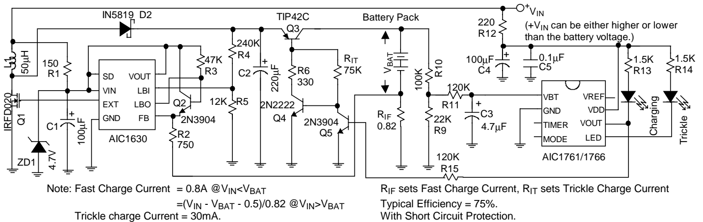
FIG. 12 Step-Up/Down Rechargeable Battery Charger
