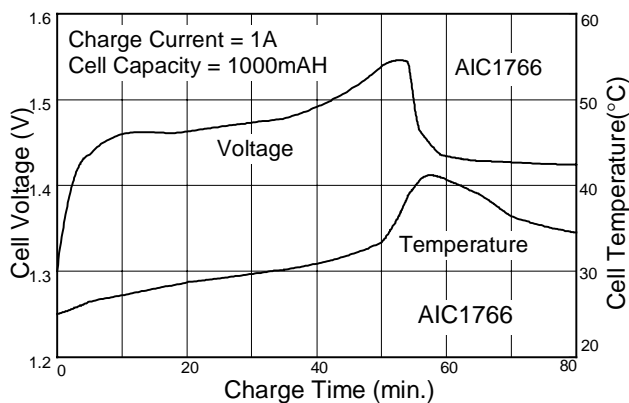
Fig. 5 Charge Characteristics of NiMH Battery
