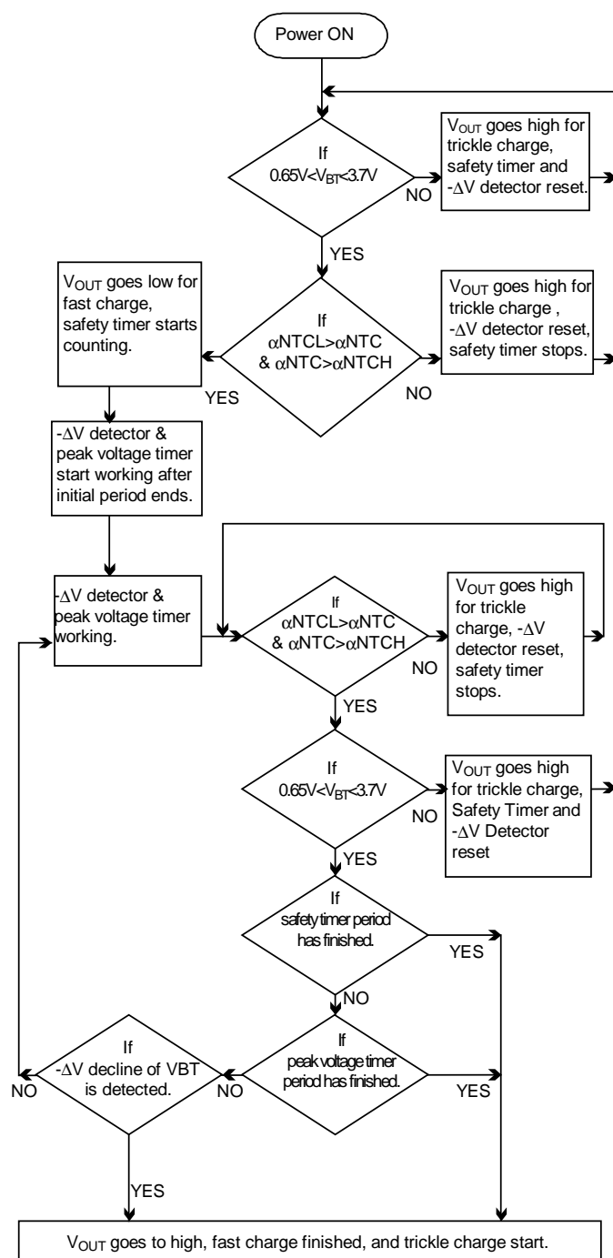
Fig. 2 Operation Chart of the AIC1761/1766
