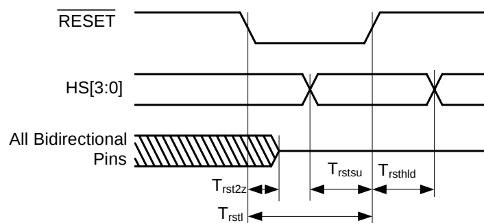
Figure 2. RESET Timing
