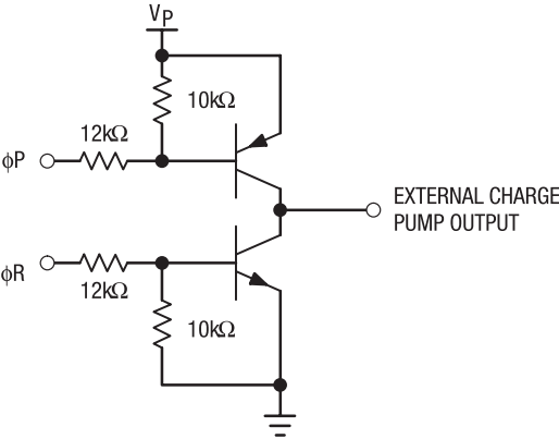
Figure 8. Typical External Charge Pump Circuit
