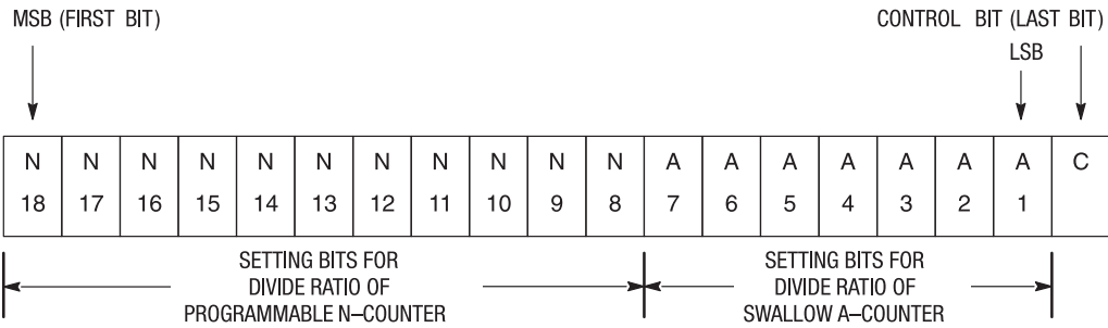
DIVIDE RATIO OF PROGRAMMABLE N-COUNTER
