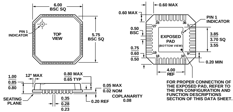
Figure 57. 36-Lead Lead Frame Chip Scale Package [LFCSP_VQ] 6mm × 6mm Body, Very Thin Quad (CP-36-1) Dimensions shown in millimeters
