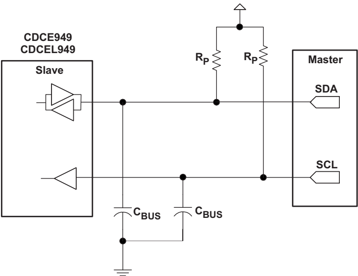
Figure 12. SDA/SCL Hardware Interface
