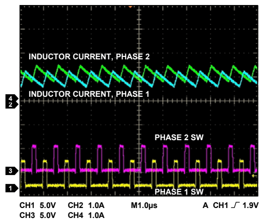
Figure 62. Combined Dual-Phase Output Operation, V_{OUT} = 1.2 \text{ V} , f_{SW} = 1.1 \text{ MHz} , 4 A Load
