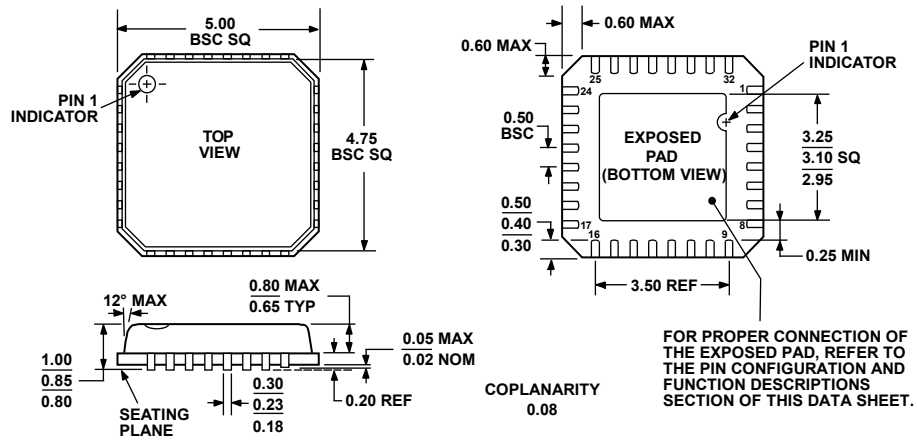
COMPLIANT TO JEDEC STANDARDS MO-220-VHHD-2 Figure 85. 32-Lead Lead Frame Chip Scale Package [LFCSP_VQ] 5 mm x 5 mm Body, Very Thin Quad (CP-32-2) Dimensions shown in millimeters
