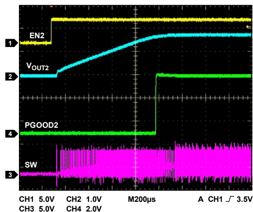
Figure 61. Power Good Signal
