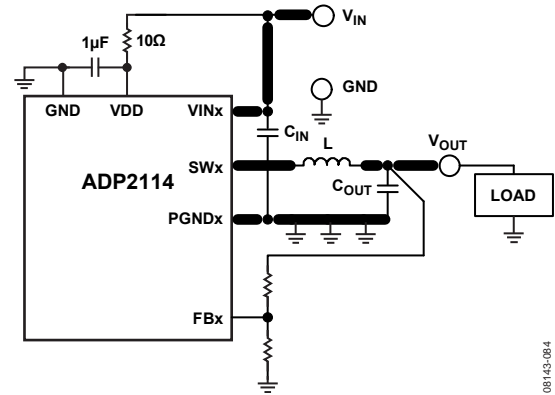
Figure 84. High Current Traces in the PCB Circuit
