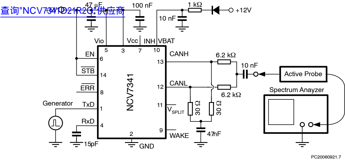
Figure 10. Basic Test Setup for Conducted Emission Measurement
