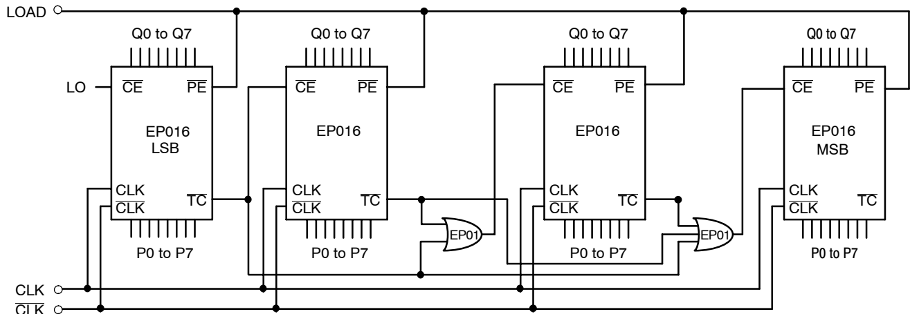
Figure 3. 32-Bit Cascaded EP016A Counter
