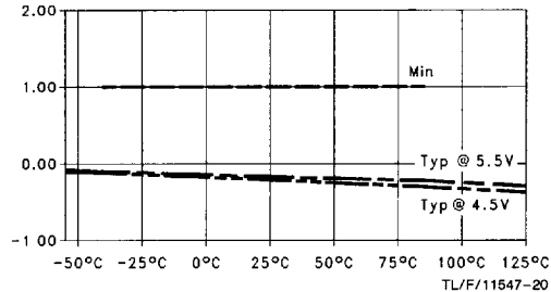
t HOLD LOW vs Temperature (T A ) C L = 50 pF, 1 Output Switching Data to LE
