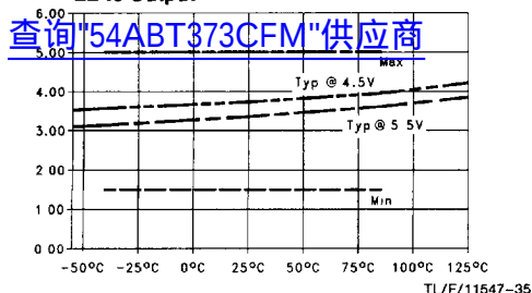
t_{PLH} vs Temperature ( T_A ) C_L = 50 pF, 1 Output Switching LE to Output
