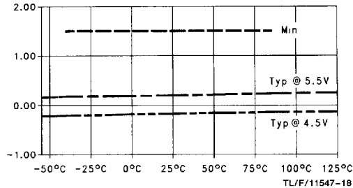
t SET HIGH vs Temperature (T A ) C L = 50 pF, 1 Output Switching Data to LE
