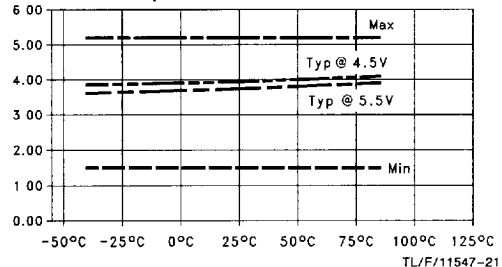
t PLH vs Temperature (T A ) C L = 50 pF, 8 Outputs Switching Data to Output
