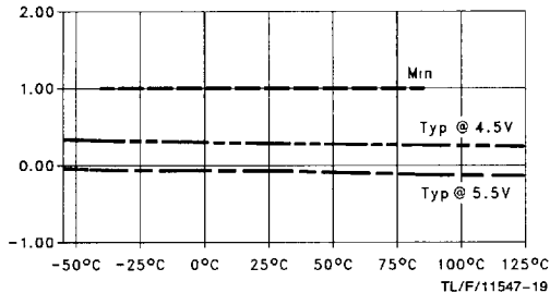
t HOLD HIGH vs Temperature (T A ) C L = 50 pF, 1 Output Switching Data to LE
