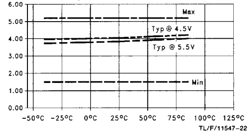
t PHL vs Temperature (T A ) C L = 50 pF, 8 Outputs Switching Data to Output
