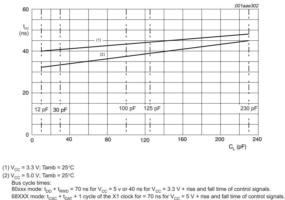
Figure 5-1. Port Timing as a Function of Capacitive Loading at Typical Conditions
