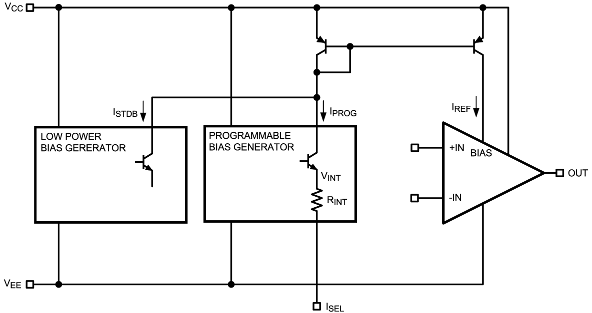
FIGURE 1. Simplified Schematic
