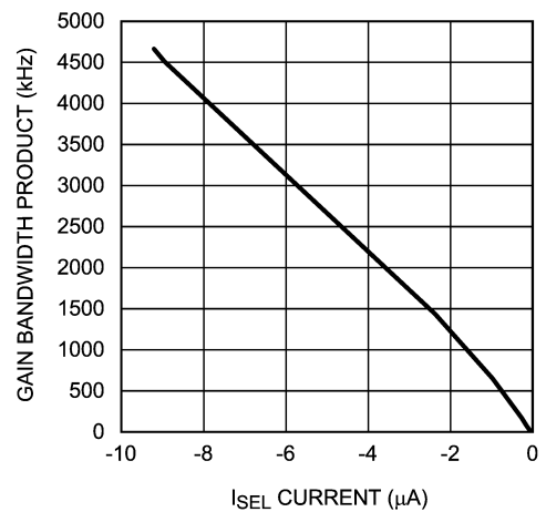
Gain Bandwidth Product vs. I_{\text{SEL}}
