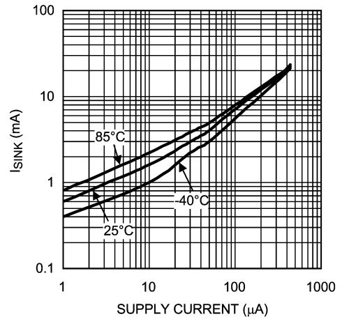
I_{\text{SINK}} vs. Supply Current
