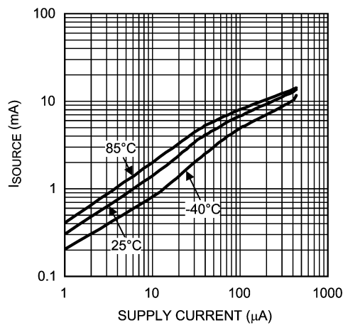
I_{\text{SOURCE}} vs. Supply Current
