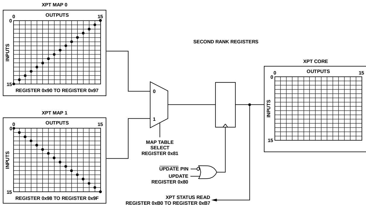
Figure 41. Crosspoint Connection Map Block Diagram
