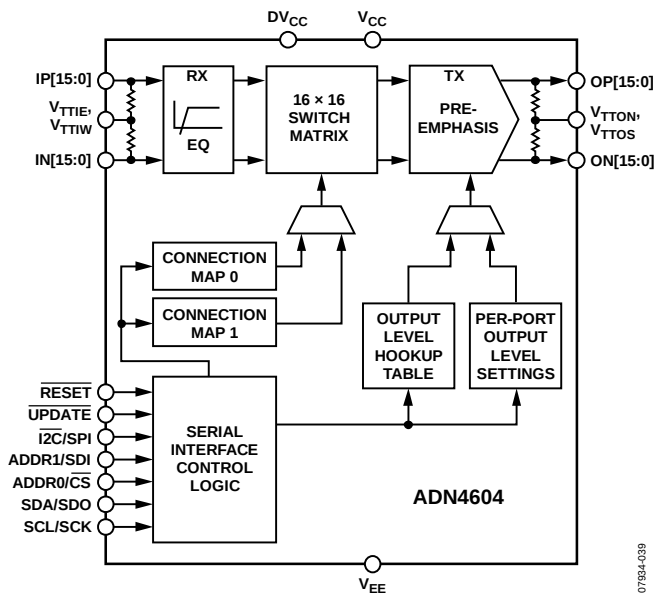
Figure 39. Block Diagram
