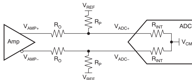
Figure 36. Resistor Network to DC Level Shift Common-Mode Voltage
