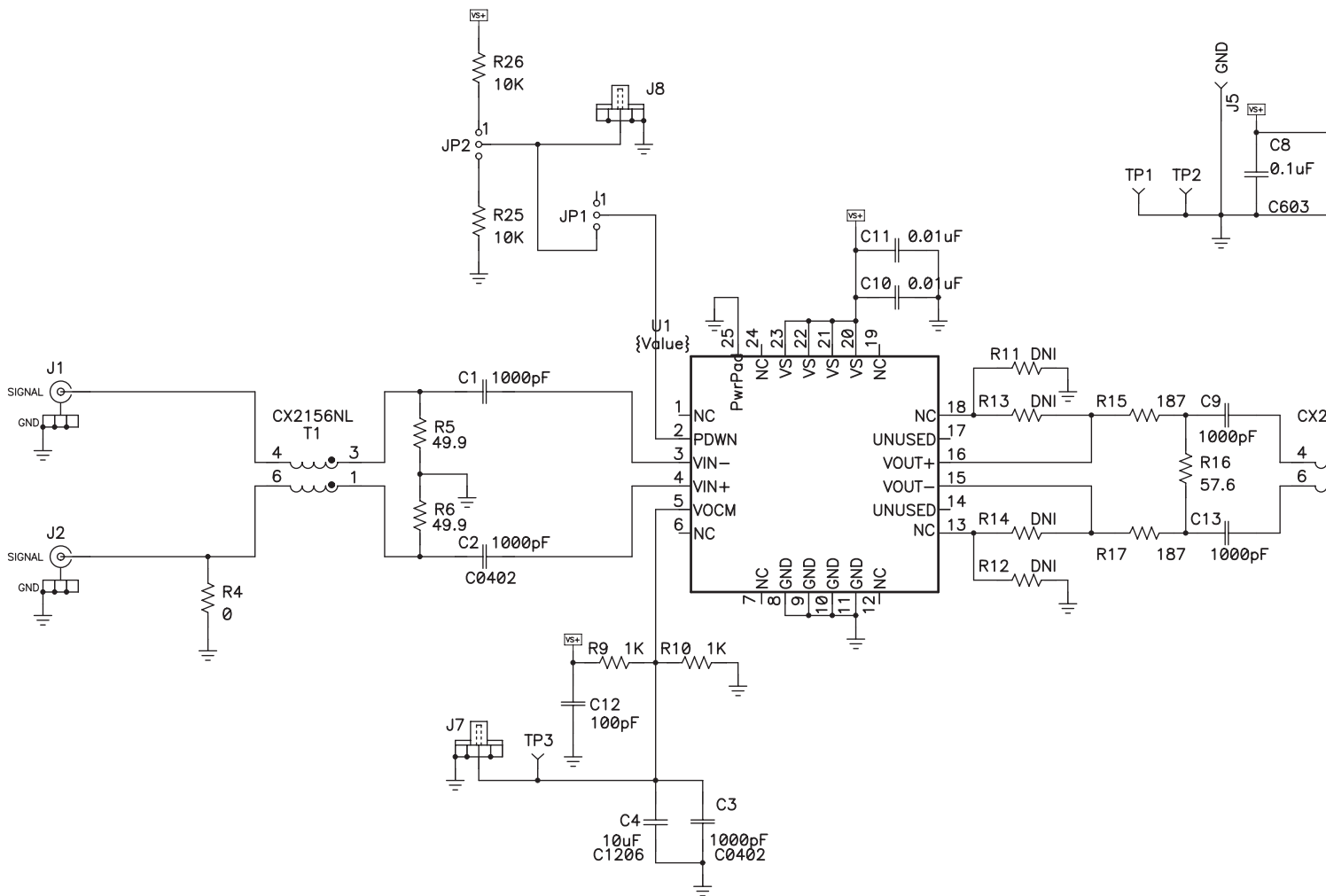
Figure 32. THS770006IRGE EVM Schematic
