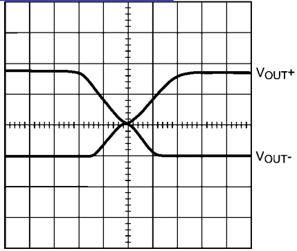
Output Transition High to Low, Low to High V_{DD} = 5V, 1V/div, 400ns/div
