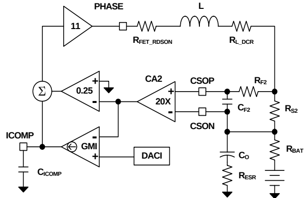
FIGURE 21. CHARGE CURRENT LIMIT LOOP
