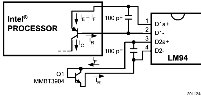
FIGURE 4. Thermal Diode Current Paths
