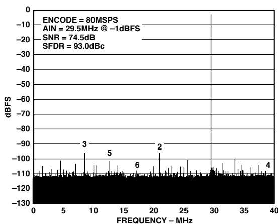
TPC 3. Single Tone @ 29.5 MHz
