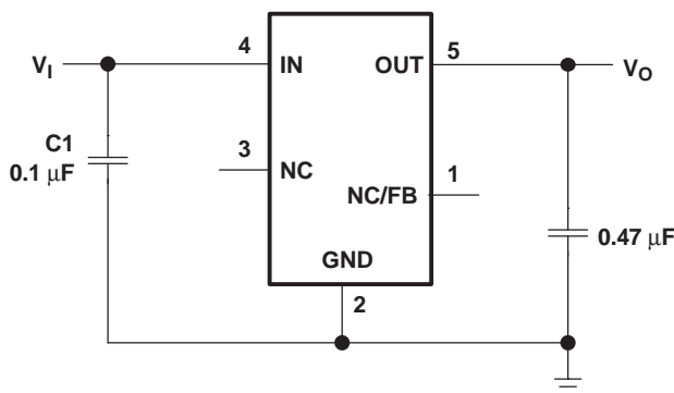
Figure 15. Typical Application Circuit (Fixed Voltage Version)
