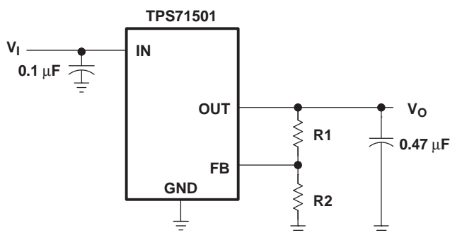
Figure 16. TPS71501 Adjustable LDO Regulator Programming
