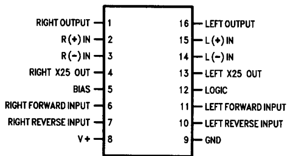
Small Outline Package
