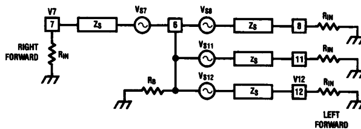
FIGURE 10. AC Equivalent of Figure 1
