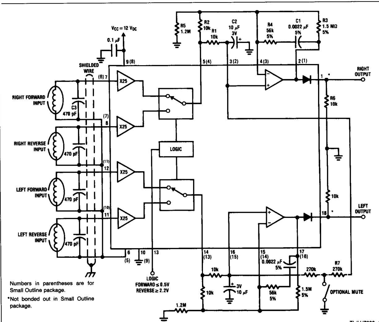
FIGURE 1. Autoreversing Tape Playback Application
