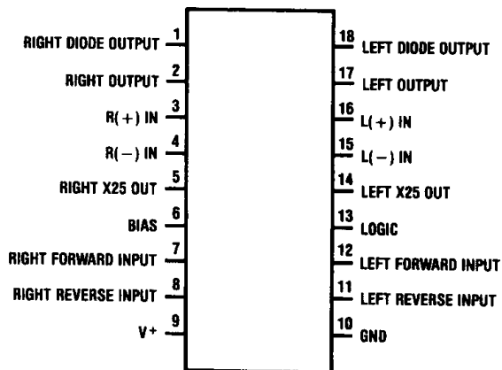
Dual-In-Line Package
