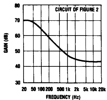
FIGURE 3. Frequency Response of Test Circuit
