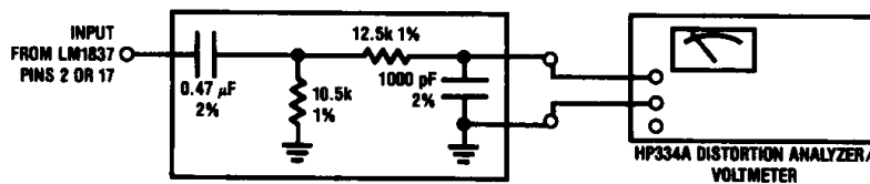
FIGURE 4. Simple 32 Hz-12740 Hz Filter and Meter
