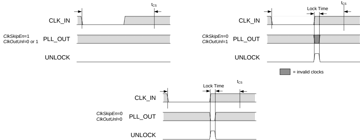
Figure 9. CLK_IN removed for < t_{CS}
