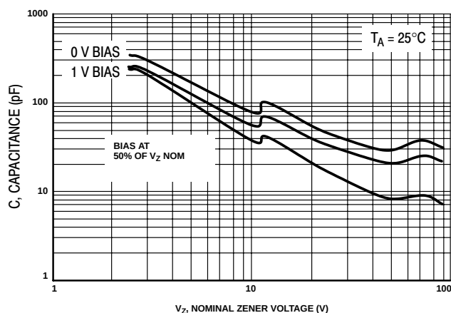
Figure 5. Typical Capacitance
