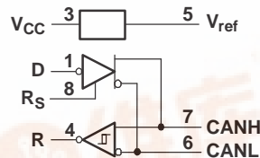
function diagram (positive logic)
