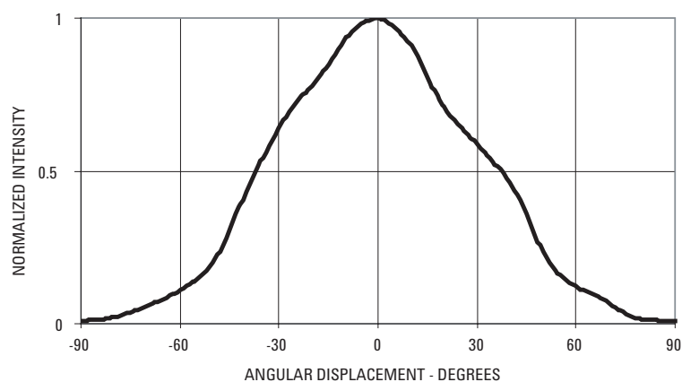
Figure 10. Spatial radiation pattern for RGB – major axis
