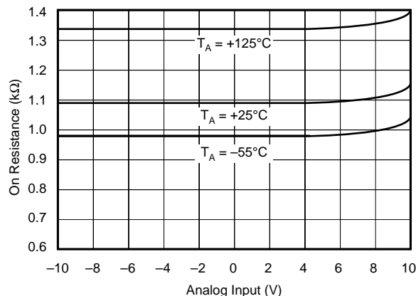
ON RESISTANCE vs ANALOG INPUT VOLTAGE
