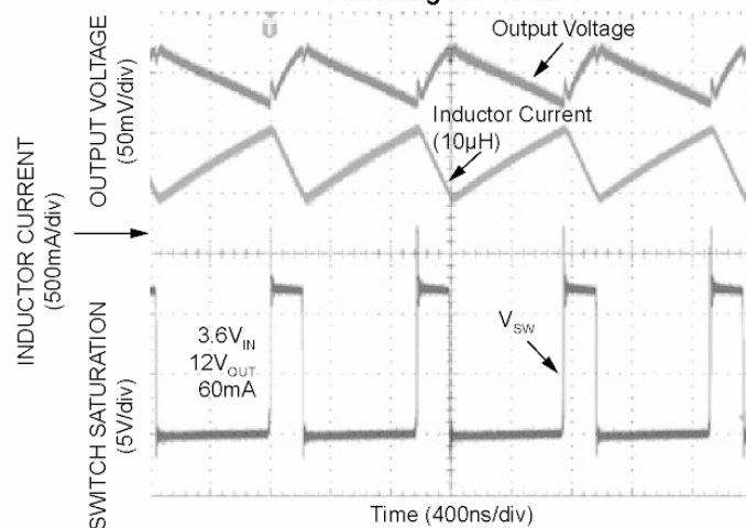
Switching Waveforms
