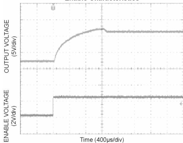
Enable Characteristics
