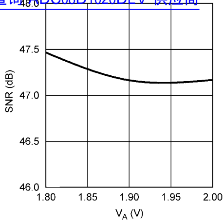
SNR vs. SUPPLY VOLTAGE 查询"ADC08D1020DEV"供应商
