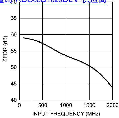
SFDR vs. INPUT FREQUENCY 查询"ADC08D1020DEV"供应商
