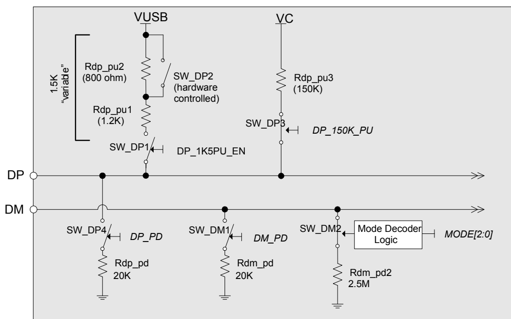
SW_DP1 is used to switch in or out the variable DP pull-up resistor, while the combination of SW_DP2, Rdp_pu1 and Rdp_pu2 determine the resistor value in different bus states.
