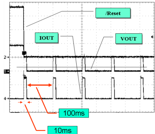
Figure 14. Buck Converter Overcurrent Protection
