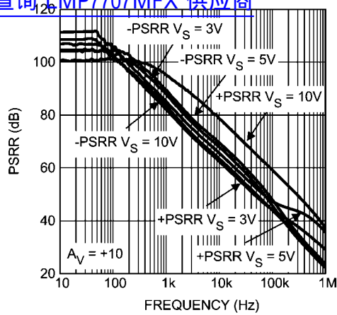
PSRR vs. Frequency 查询"LMP7707MFX"供应商
