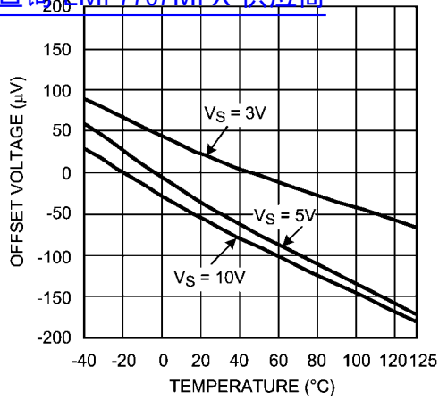
Offset Voltage vs. Temperature 查询"LMP7707MFX"供应商
