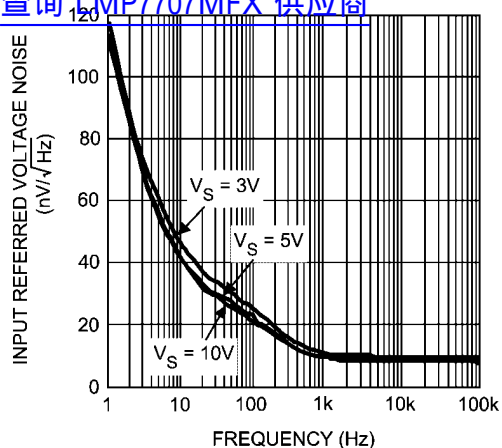
Input Voltage Noise vs. Frequency 查询"LMP7707MFX"供应商
