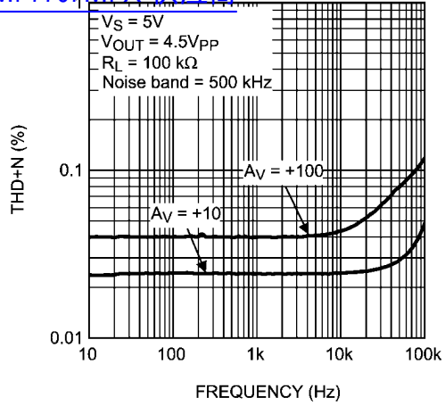
THD+N vs. Frequency 查询"LMP7707/MEX"供应商
