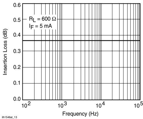
Figure 13. Insertion Loss vs. Frequency
