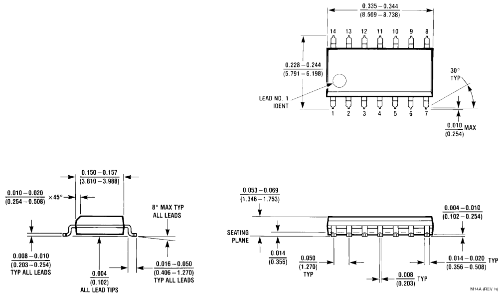
14-Lead (0.150" Wide) Molded Small Outline Package, JEDEC Order Number NM95HS01M14 or NM95HS02M14 NS Package Number M14A
