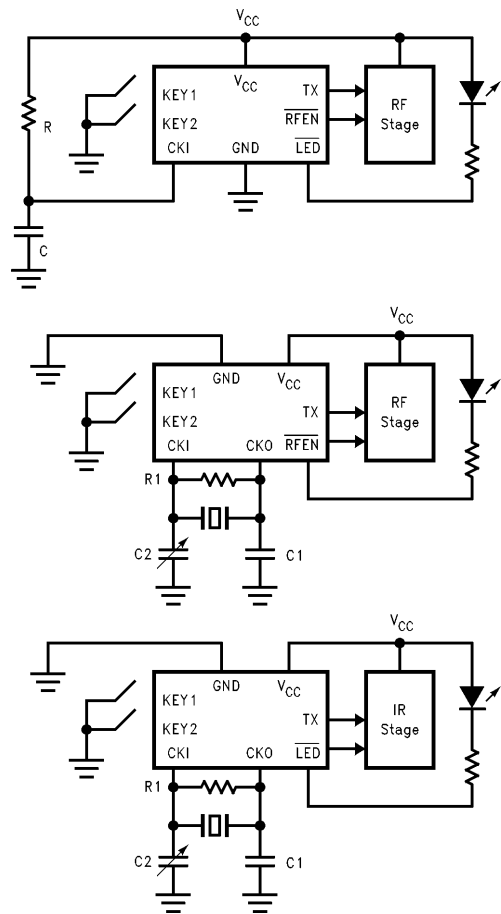
FIGURE 3. Typical Transmitter Circuit Configurations
