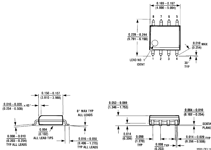
8-Lead (0.150" Wide) Molded Small Outline Package, JEDEC Order Number NM95HS01M8 or NM95HS02M8 NS Package Number M08A
