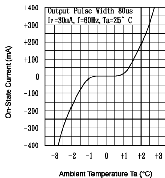
Fig.7 On-State Characteristics
