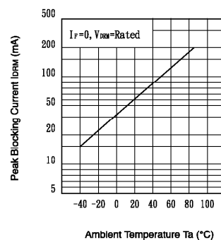
Fig.8 Leakage with LED off vs. Ambient Temperature
