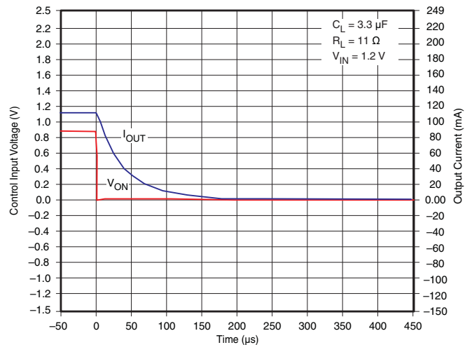
Figure 33. t_{OFF} Response
