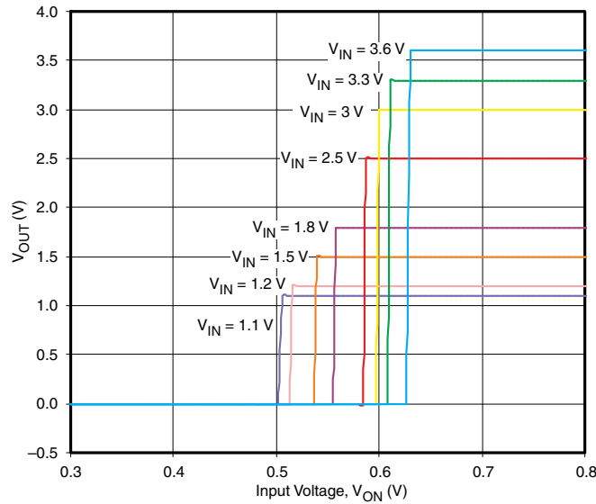
Figure 11. ON-Input Threshold
