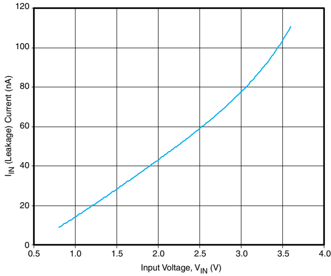
Figure 9. I_{IN}(\text{Leakage}) vs V_{IN} ( I_{OUT} = 0 )
