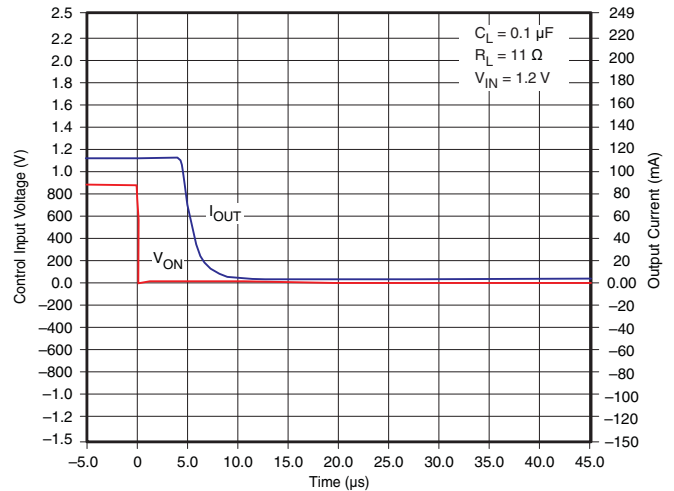
Figure 31. t_{OFF} Response
