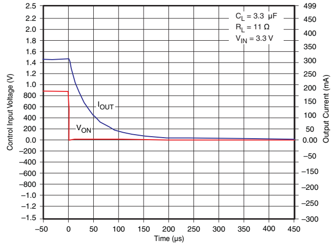
Figure 29. t_{OFF} Response
