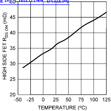
High-Side FET Resistance vs. Temperature 查询"LM20144"供应商
