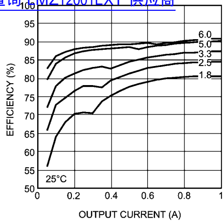
Efficiency 20V Input @ 25°C 查询LMZ12001EXT"供应商"
