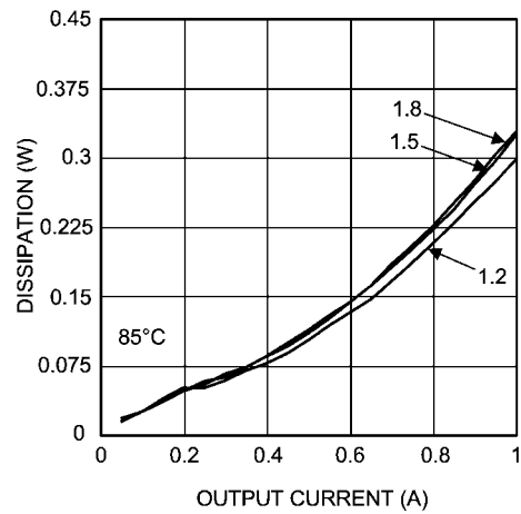
Dissipation 5V Input @ 85°C
