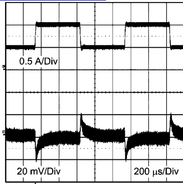
Transient Response 12VIN 3.3VOUT 0.5A to 1A Step 查询"LMZ12001EXT"供应商
