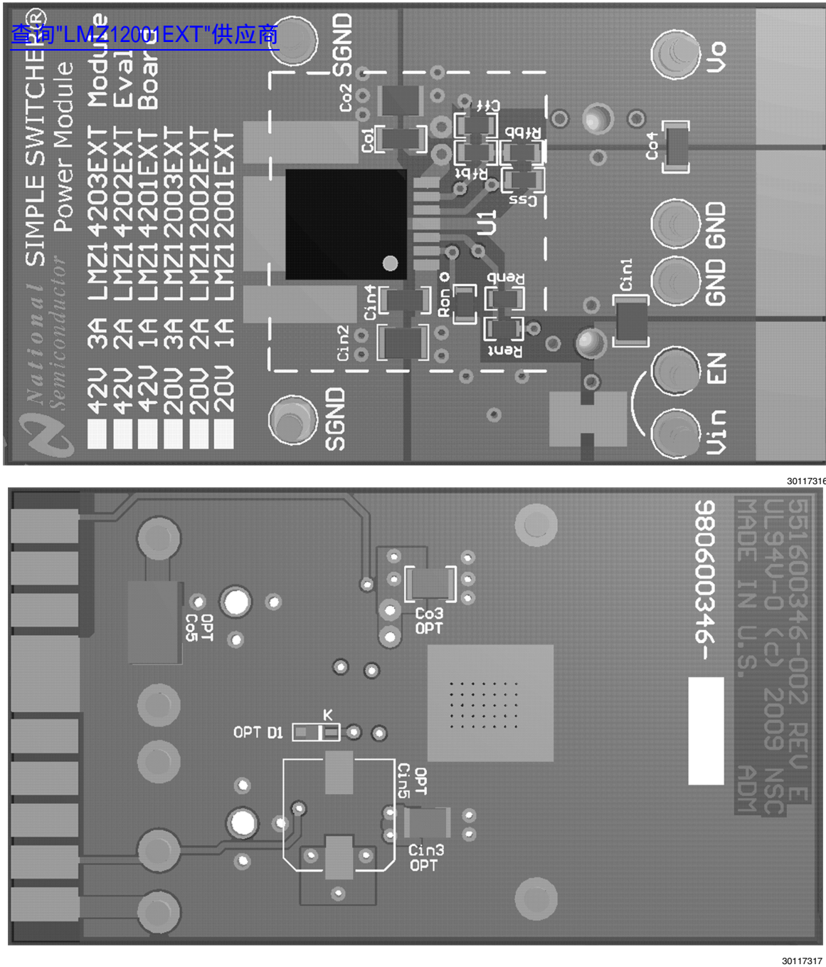
FIGURE 1. Top and bottom view of evaluation PCB
