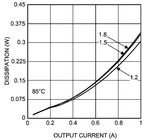
Dissipation 4.5V Input @ 85°C
