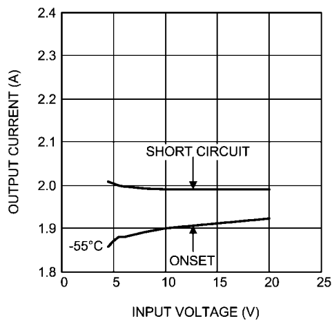
Current Limit 1.8V OUT @-55°C
