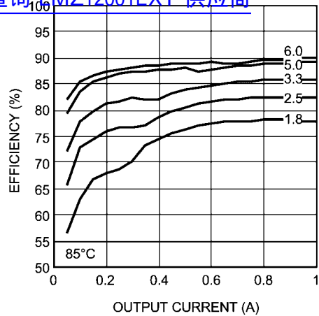
Efficiency 20V Input @ 85°C 查询"LMZ12001EXT"供应商
