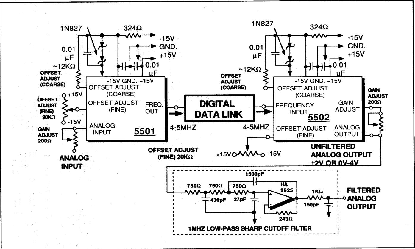
Figure 2. Typical Interconnection Scheme
