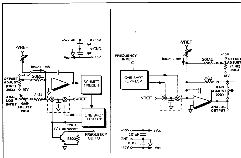
Figure 1. 5501/5502 Block Diagram
